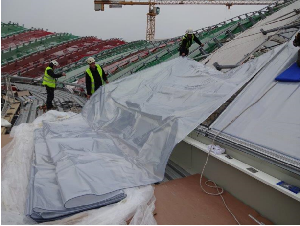
Figure 15- Installation of ETFE cushion
