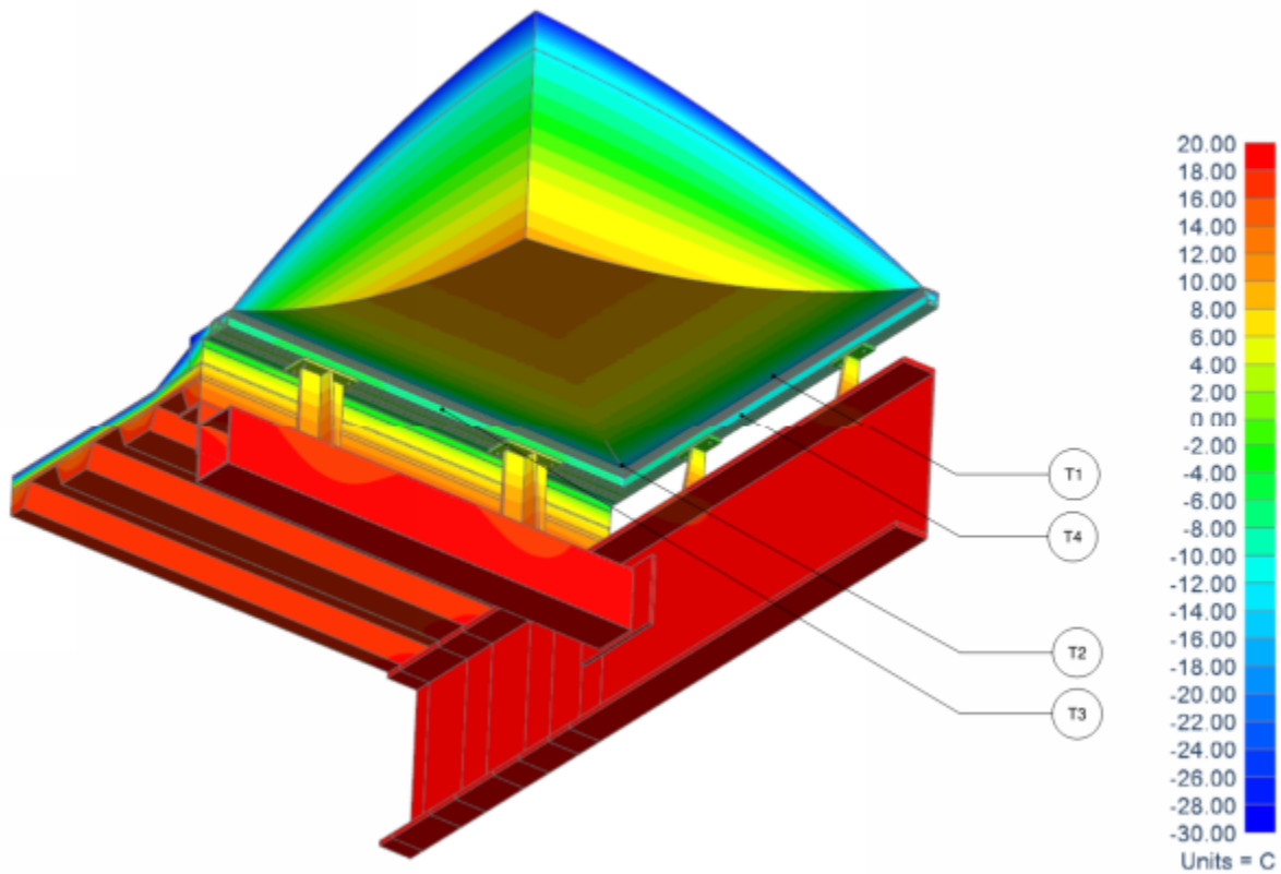
Figure 7- 3D Thermal model of 3 foil ETFE cushion in a northern climate at -22°F (-30°C)
